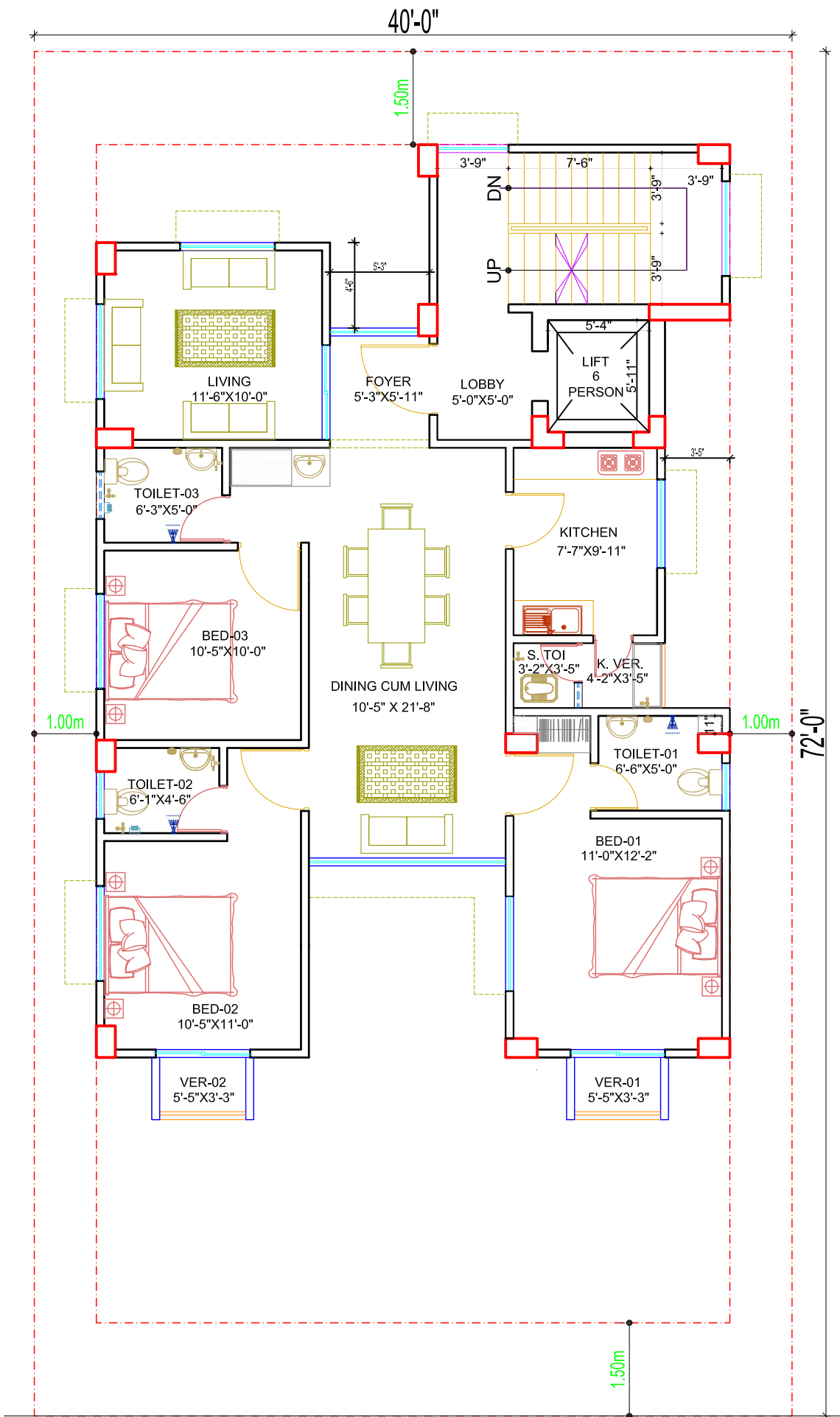
G+8 TYPICAL FLOOR PLAN
